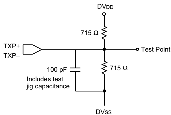
TXP Switching Test Circuit
